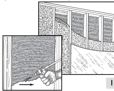
Figure 7: Flash and batt (1/2"-1" thickness)
