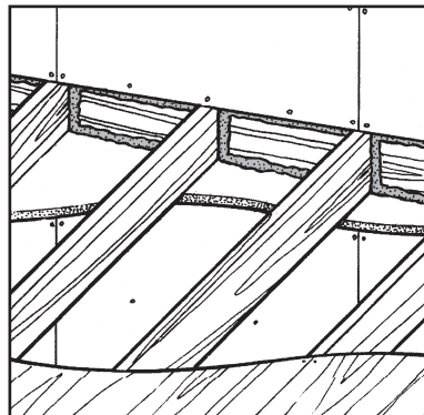
Figure 2: Sealing wall-ceiling joints
